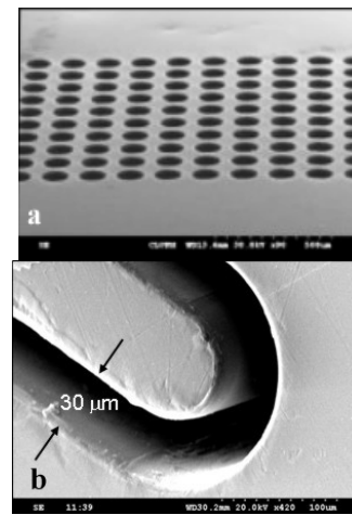
Fig. 5. Precision microfabrication: a. lattice of micro-holes made in polymeric material b. polycarbonate cutting, 1 mm thickness.
