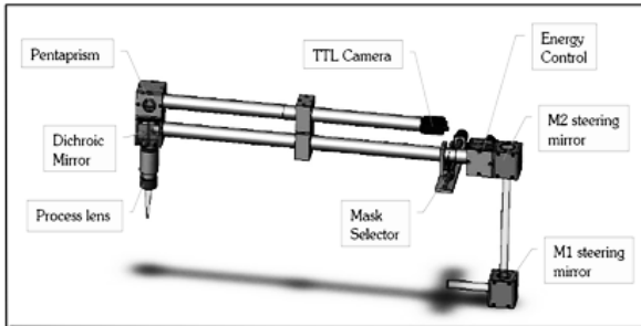
Fig. 3. ML-100 micromachining station: excimer laser path.
